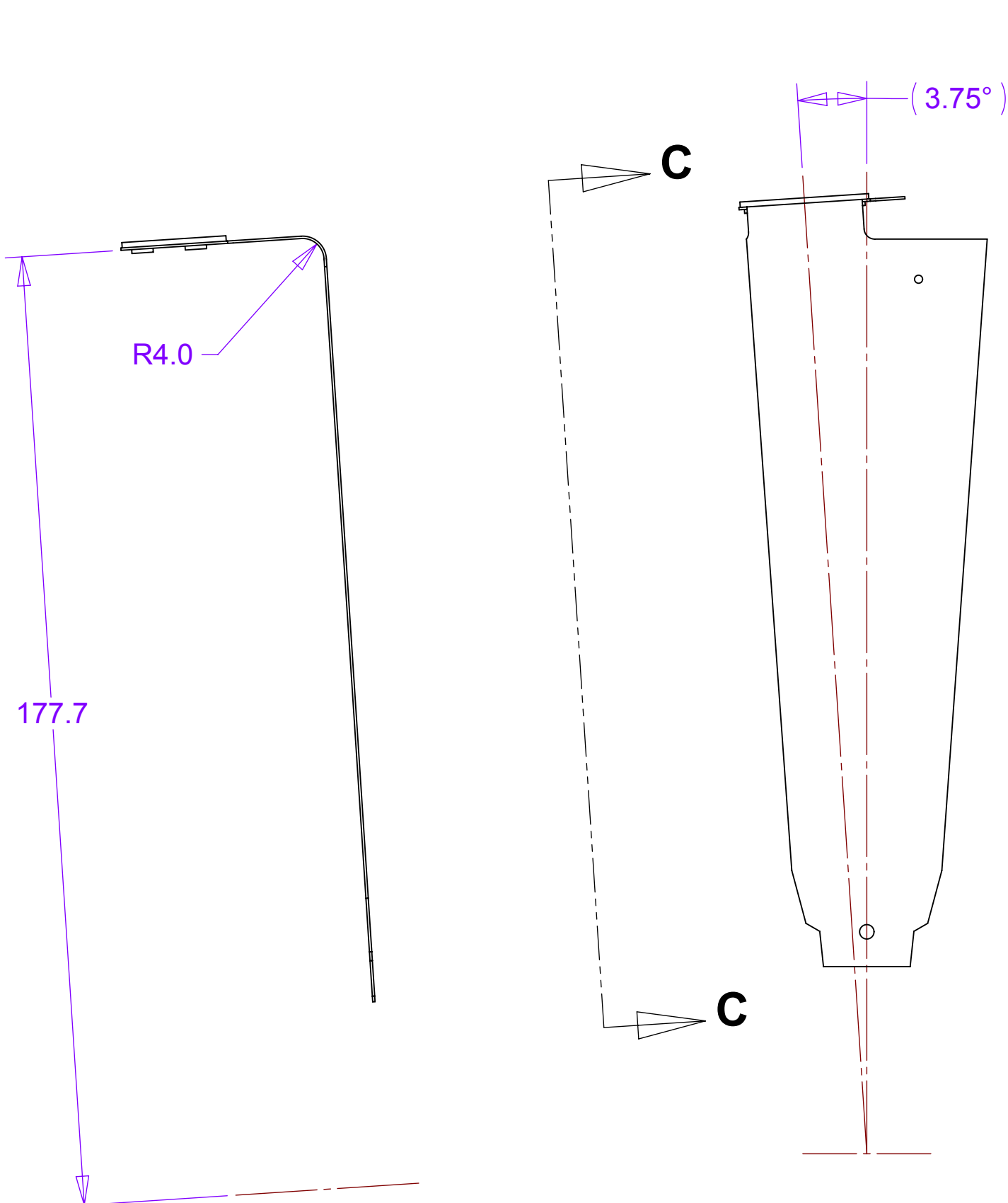
SECTION C-C
