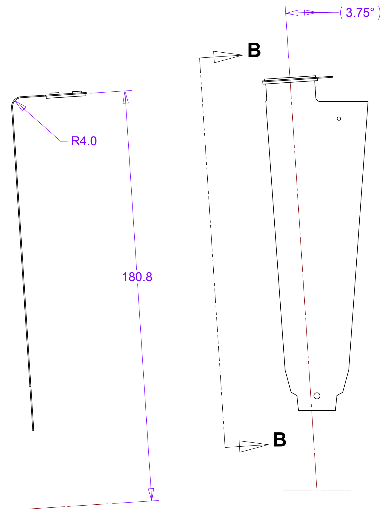
SECTION B-B
